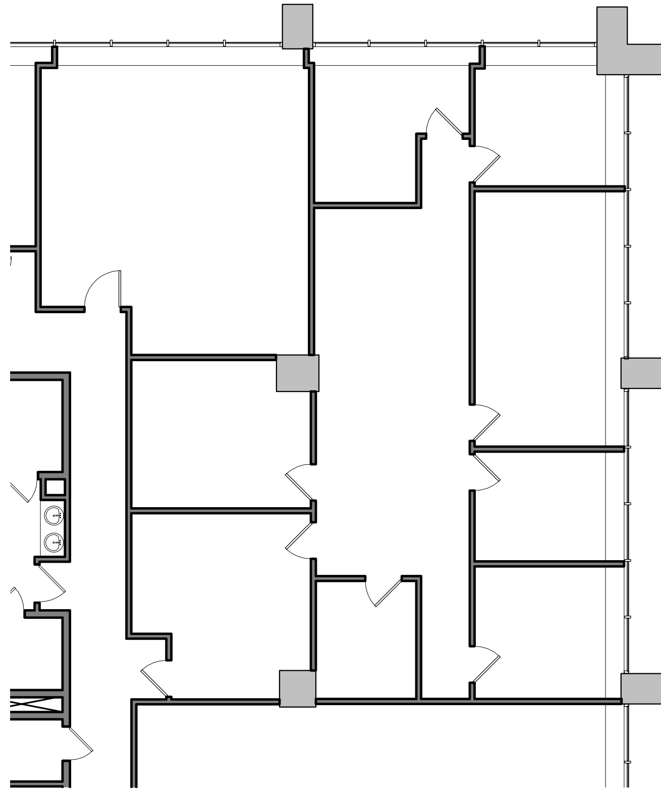
FLOOR PLAN
